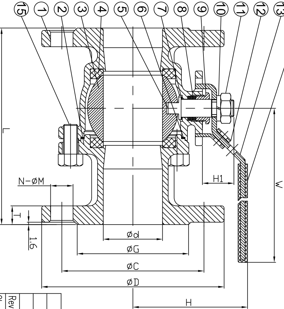
TYPE 2 21/2"-4"
